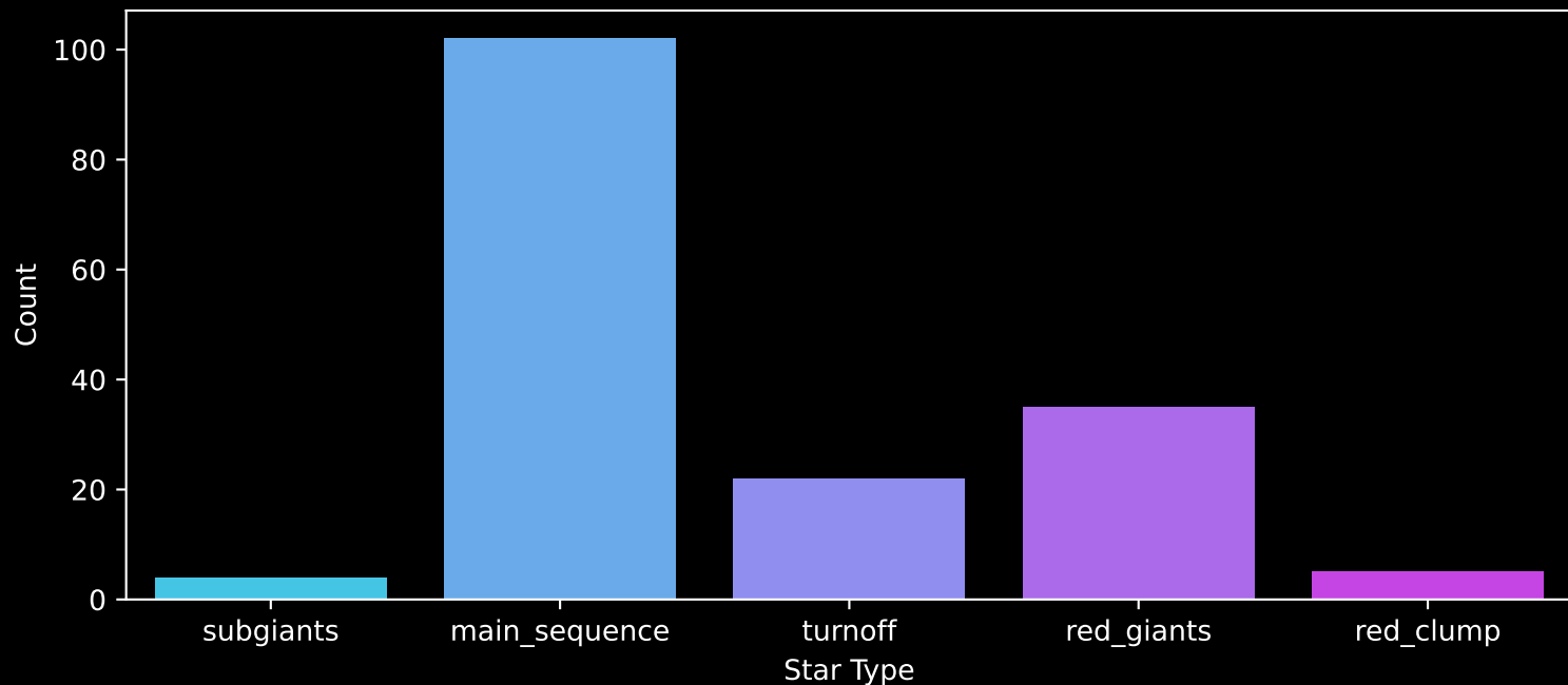
APOGEE DR17 Field: [089+70] Count plot of Star Type
