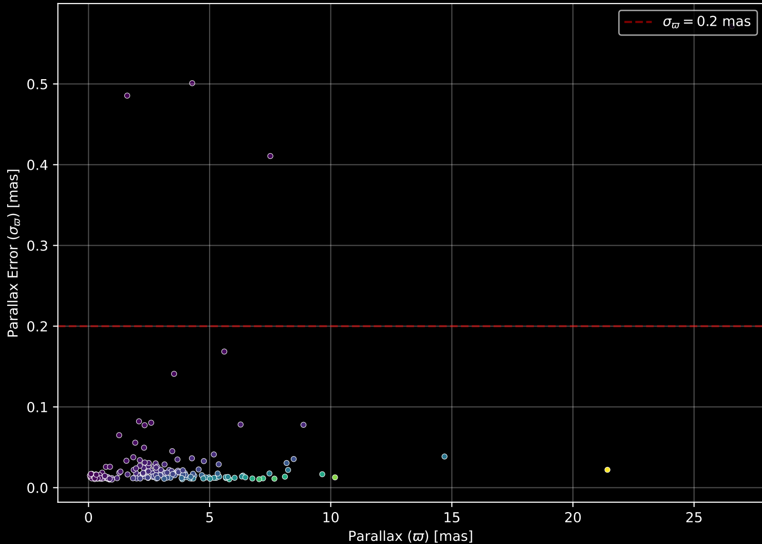
APOGEE DR17 Field: [089+70] Parallax Quality (n= 168)
