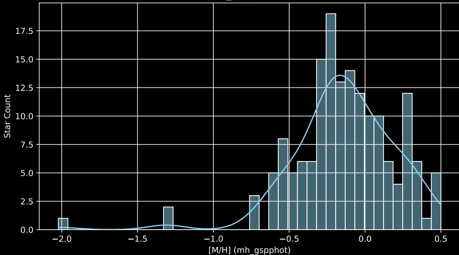
APOGEE DR17 Field: [089+70 [M/H] (mh_gspphot) (n= 163)
