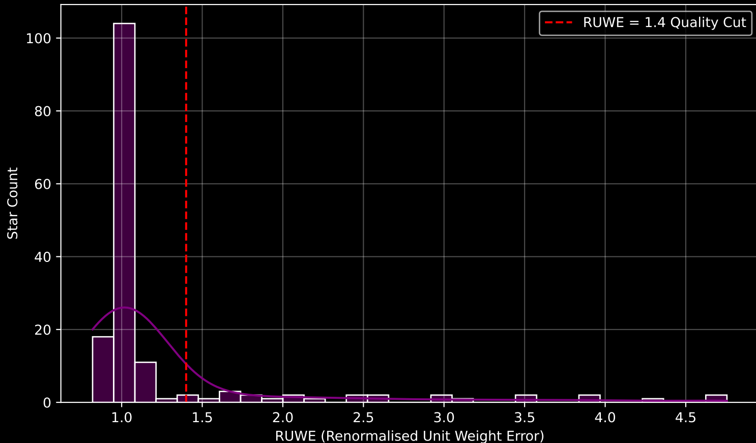
GAPOGEE DR17 Field [089+70] RUWE Distribution (n= 160)
