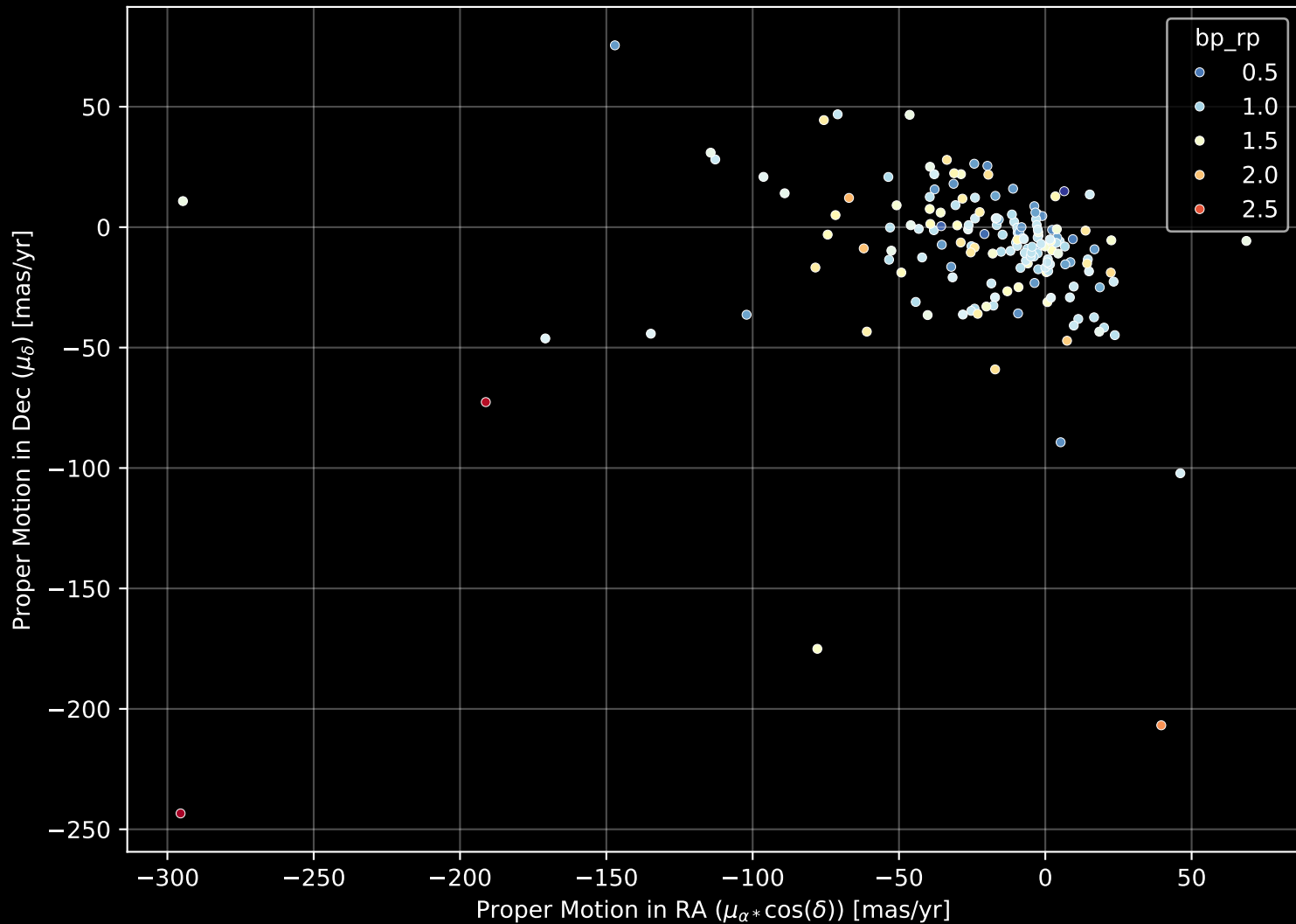
APOGEE DR17 Field: [089+70] Proper Motion Diagram (n= 168)
